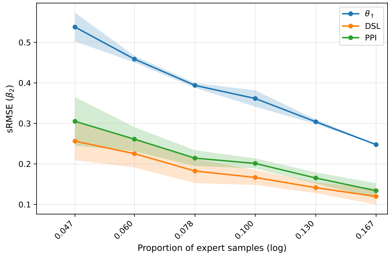
Low-Variance Feature — sRMSE \beta_2 averaged over LLMs (CUAD)
